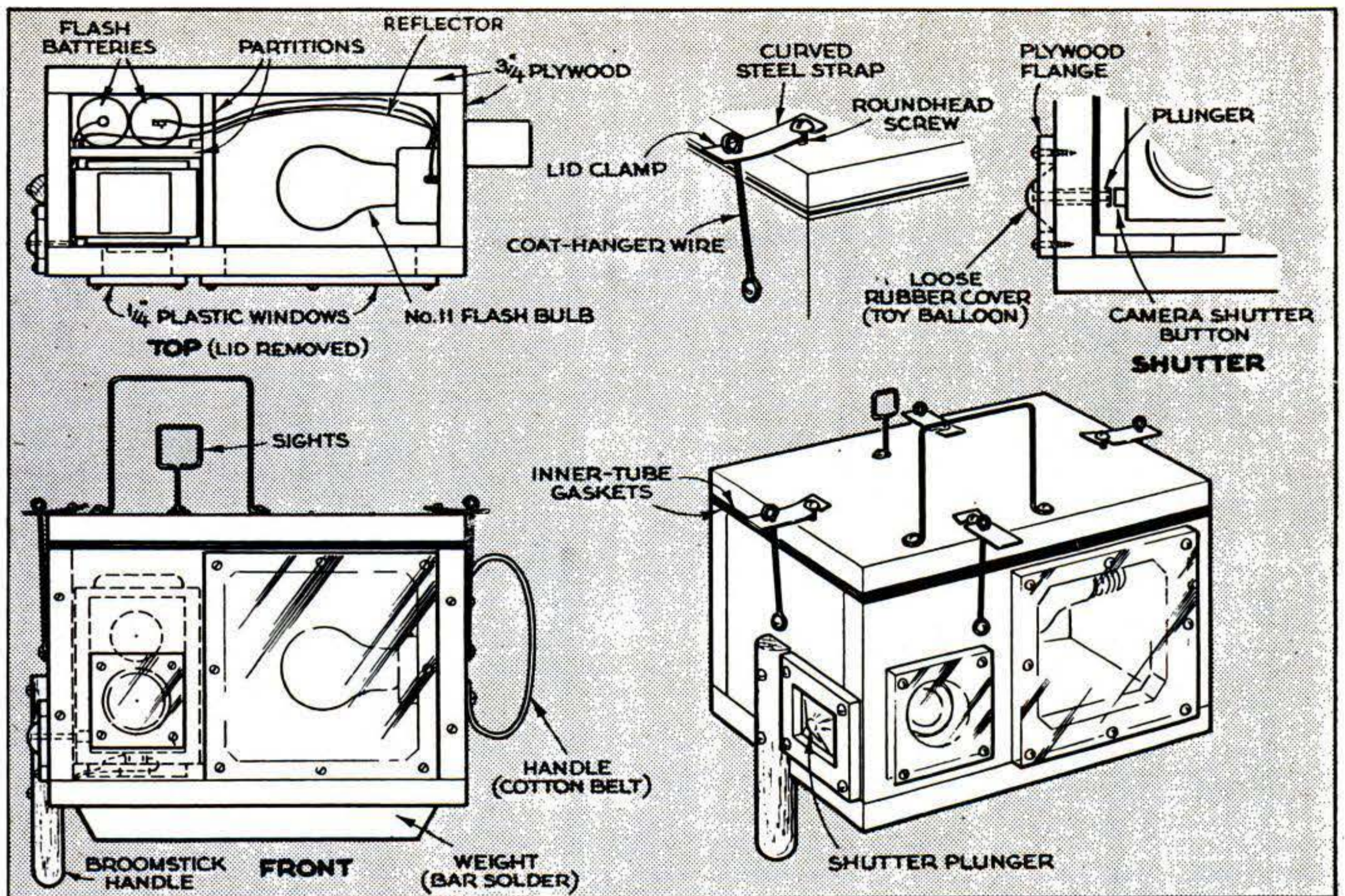
Safe inside a watertight box, the camera and flash are tripped by a rubber-sealed plunger.
